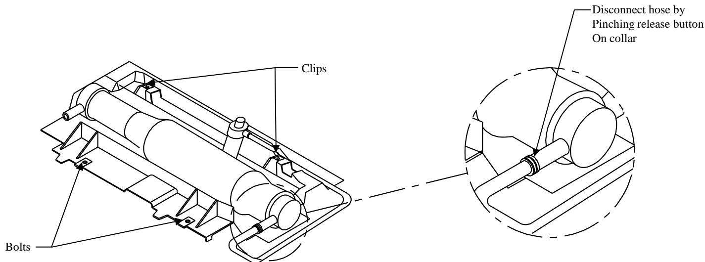
Figure 2 Carbon Canister
