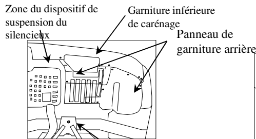
Figure 1. Cadre-support de suspension
