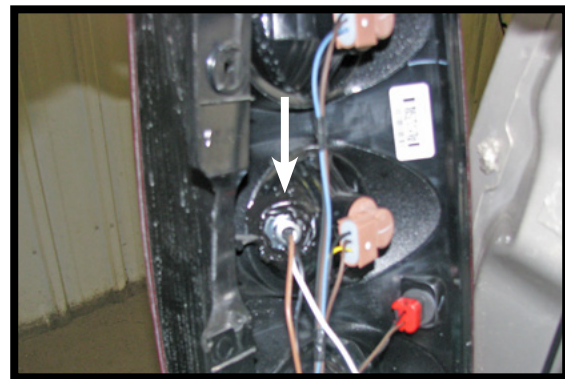
Possible locations for the BX8869 wiring kit. Location can vary depending on model of vehicle.
