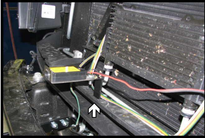
13. If installing a breakaway, attach the bracket to crossmember using 1/4"-20 x 3/4" bolt, 1/4" flat washer and 1/4"-20 nut.
