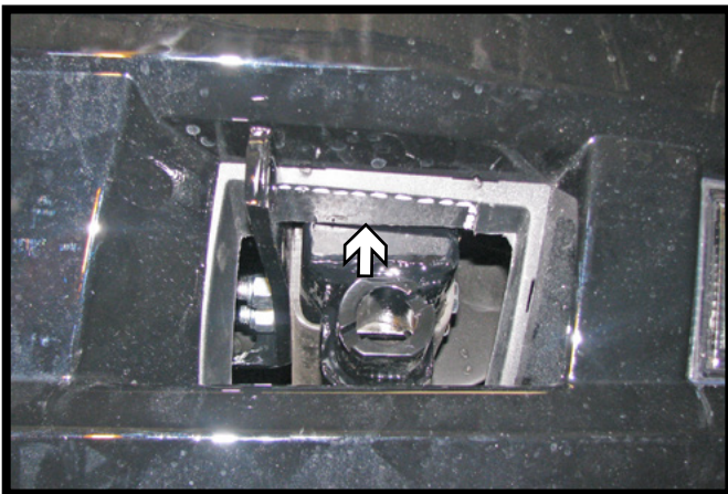
15. Some models may require additional trimming of the upper tow hook pocket to allow for baseplate clearance.
