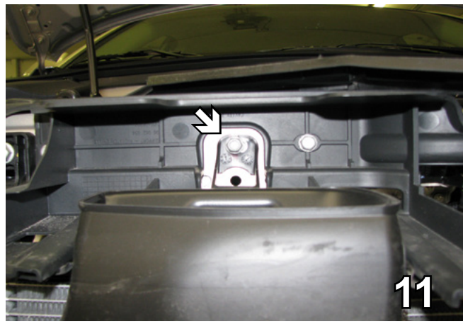
11. Using a 10MM socket, remove the metric bolt from the top of the air intake tube. Set the bolt and the tube aside to be reinstalled later.
