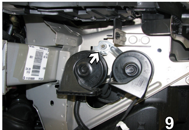
9. Using the 13MM socket, remove the metric bolt from the horn bracket on the driver's side, unplug and set the bolt and horn aside to be reinstalled later.
