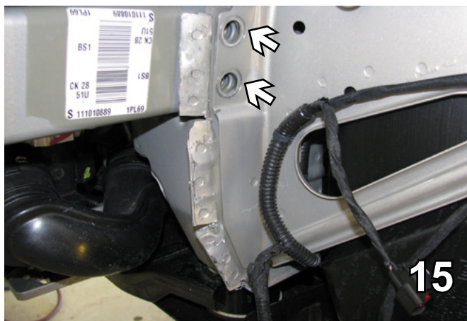
15. Using an 18MM socket and a wrench on the other side, remove the two metric bolts next to the flattened area. Do this on both sides. Set bolts aside to be reinstalled later.
