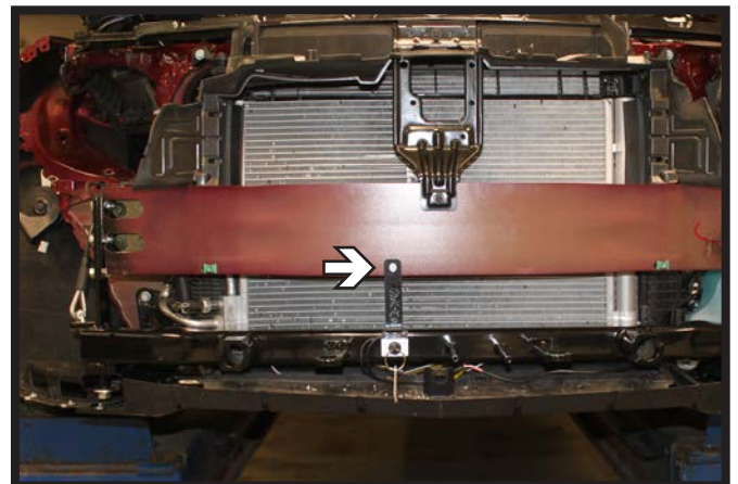
18. Optional Breakaway: In the desired location, drill a 1/4" hole thru the bumper lip. Install the bracket to the bumper with the provided 1/4" hardware. Attache the breakaway to the bracket with the 1/4" hardware provided.
