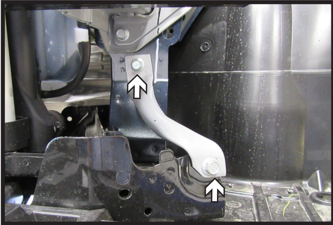
12. Using a 14MM socket, remove the two (2) bolts, and remove the brace.
