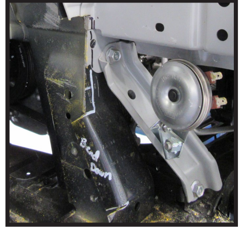
14. On the passenger side, measure down from the top of the frame extension 3" and mark. Mark out a notch from the 3" mark down to the bend flush with the inner frame side. Further down, make a mark at the bottom of the bend as deep as the upper notch (gray). Using a reciprocating saw, cut the bottom line (gray) and the bottom side of the upper notch. Bend the lip back towards the frame. Continue cutting out the upper notch flush to the inner frame. Treat the driver side similarly, starting just below the lower bolt. A completed picture of the passenger side is pictured.
