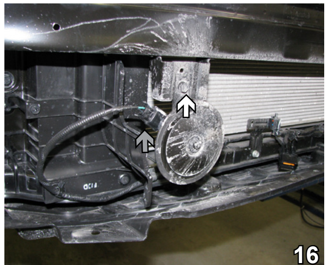
16. Using the 10MM socket, remove the bolt from the horn bracket (white). Disconnect the wiring and set the horn aside (gray).
