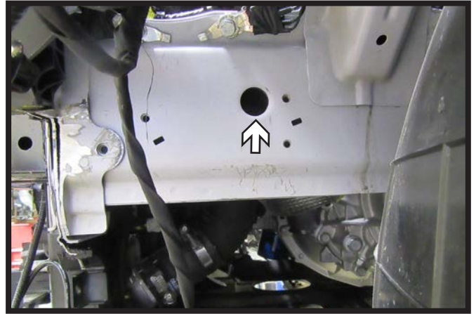
15. Using a 1-1/4" drill bit, drill an access hole as indicated into the side of the frame. Do this on both sides of the vehicle.
