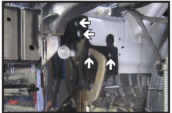
17. Using a 3/8" drill bit, drill the remaining four (4) holes on the baseplate. Do this on both side of the vehicle.
