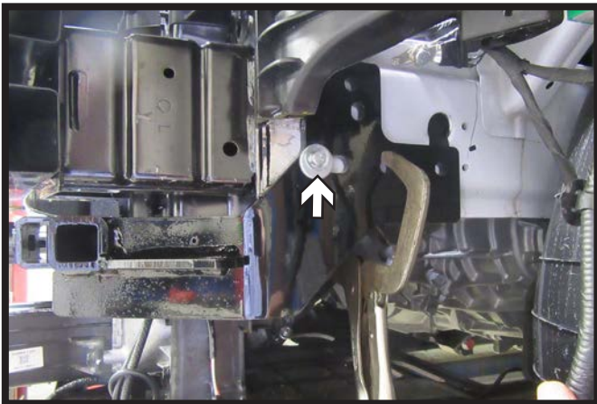
16. Slide the baseplate into position and line up with the existing hole on side of the vehicle. Make sure the baseplate is level. Clamp into place. Insert one (1) 6MM bolt. Do this on both sides of the vehicle.
