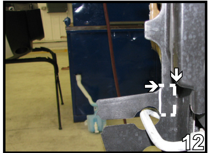
12. On the passenger side, remove the top part of the plastic flap by cutting with a utility knife straight down above the hose. Notch out a little farther by cutting in as far as you can.
