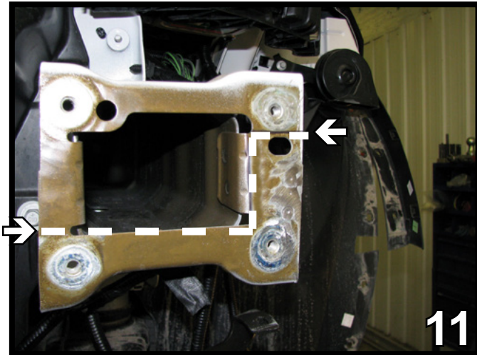
11. On the top outside of each bumper end, cut across at the bottom of the groove, straight down on the outside of the frame rail, across the bottom flush with the front of the frame and remove the whole piece. Do this on both sides.
