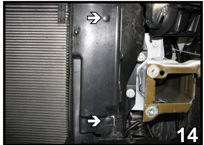
14. Remove the two push pins holding the plastic cover. Do this on both sides. Set the push pins and plastic aside to be reinstalled later.
