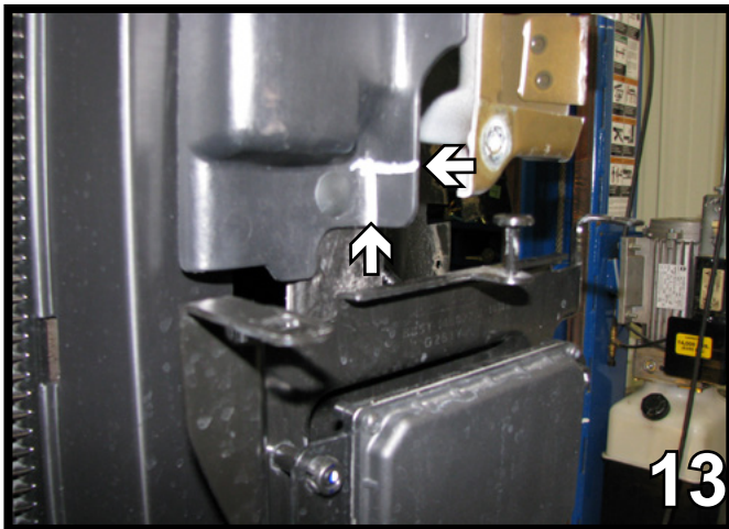
13. On the driver's side, cut a little square notch out of the corner of the plastic air dam with a utility knife.
