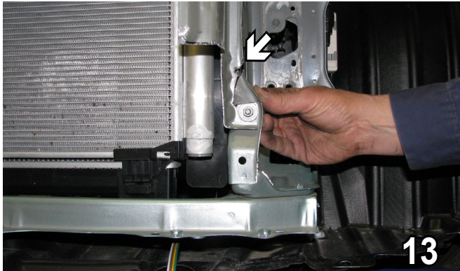
13. Using a reciprocating saw, cut above the bolt in the frame horizontally and then diagonally up and remove the notch. Do this on both sides.
