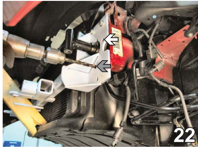
22. Using the baseplate as a template, drill two holes into the frame end using a 13/32" drill bit. From the backside of the baseplate, insert a 3/8-16 x 1 1/4" hex bolt and fasten to the 3/8" lock washer and 3/8-16 hex nut (grey arrow). From the front side of baseplate, insert a 3/8-16 x 1 1/4" hex bolt and fasten to the 3/8" lock washer and 3/8-16 hex nut (white arrow). Do this to both sides of the vehicle.
