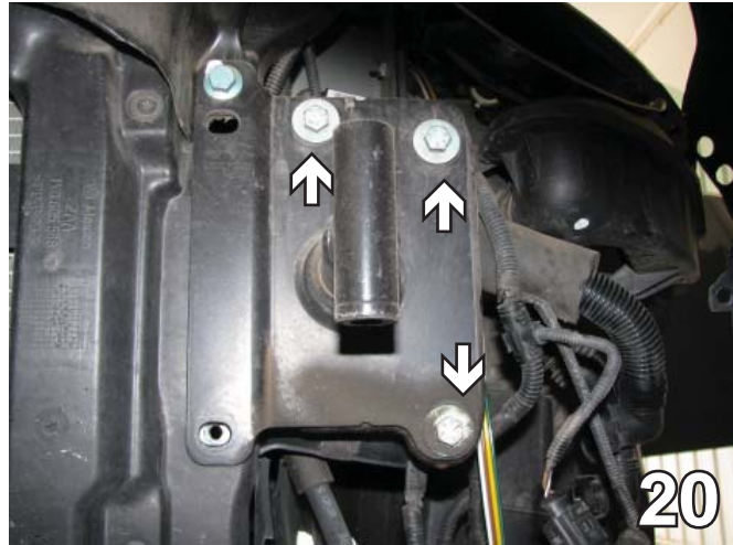
20. Using a 13MM socket, remove the three bolts from the bumper bracket on the driver's side. On the passenger side remove the top two bolts. There is no bolt in the bottom hole.
