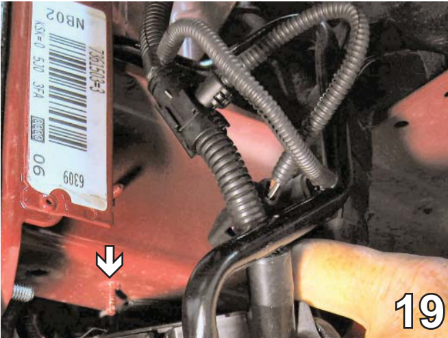
19. On the driver's side, pull down on the coax housing to separate it from the pin attached to the underside of the frame rail. Using a flat cold chisel, cut off the pin. This will prepare the area for installation of plate later.
