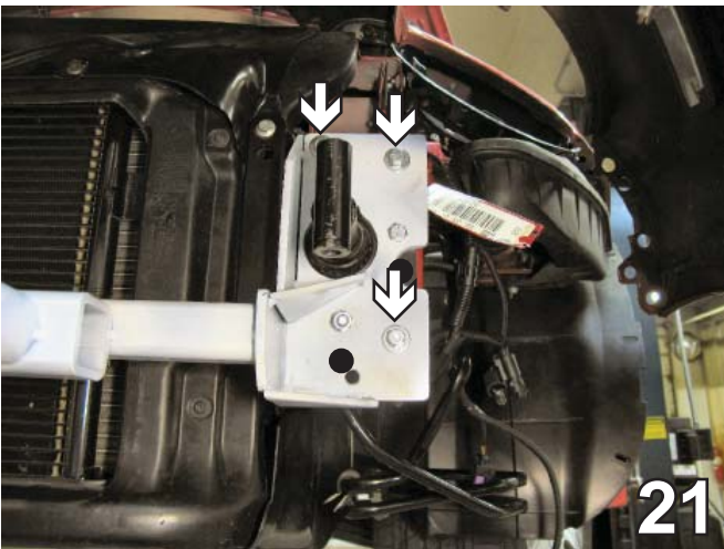
21. Slide the baseplate over and encircling the bumper bracket. Align the baseplate with the three existing holes of the bumper bracket (white arrows). Insert the 8MM-1.25 x 30MM hex bolts and fasten to the 5/16" lock washers and 5/16" flat washers to these bolt locations. Do this to both sides of the vehicle. Baseplate painted white to enhance visibility.
