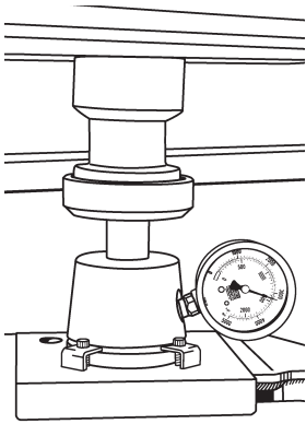
FIGURE 7—Gauge showing 3,000 lbs.
